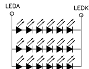
CONSTANT CURRENT:60mA,18.6V(REF.) BACKLIGHT DRIVER CIRCUIT DIAGRAM
